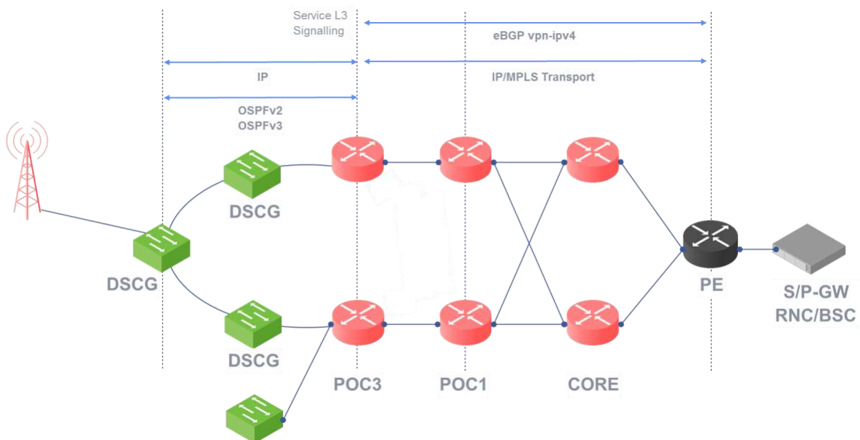
Figure 10. Scenario 1: Dual-home IP/MPLS Ring
