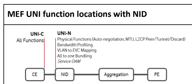
Figure 6. MEF UNI functional delivery model with DCSG working as Enterprise NID
