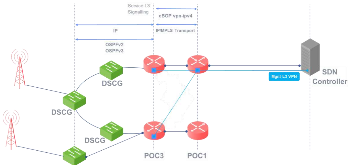
Figure 16. Auto Configuration in IP/MPLS Networks
